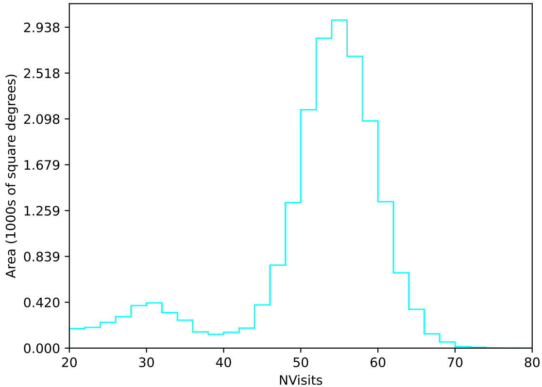
ddf_loaded_fl2_v3.4_10yrs All sky u band: NVisits
