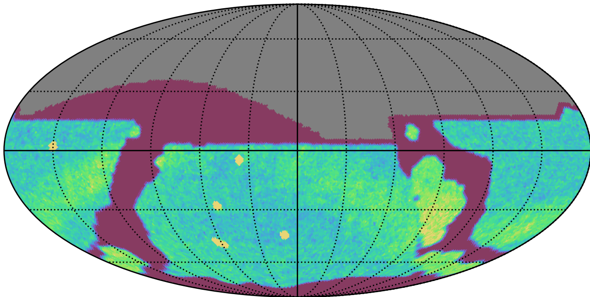
ddf_loaded_fl2_v3.4_10yrs All sky r band: NVisits
