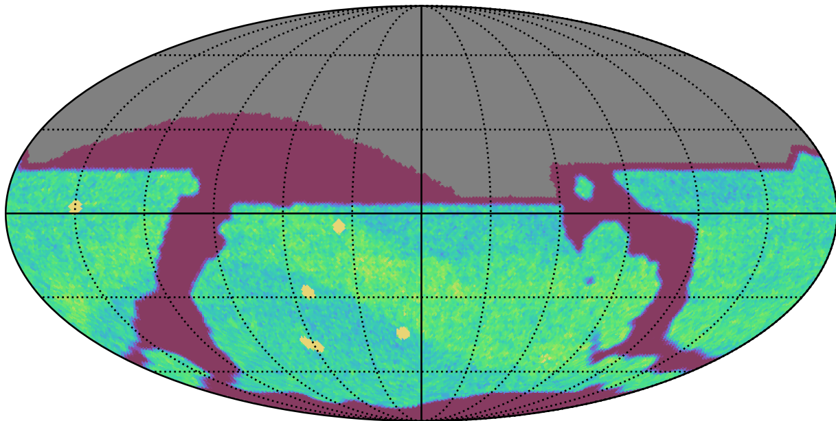
ddf_loaded_fl2_v3.4_10yrs All sky i band: NVisits
