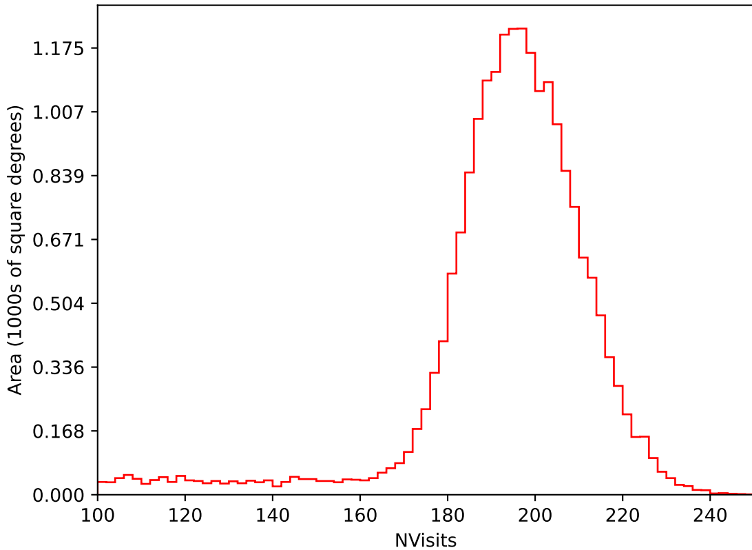
ddf_loaded_fl2_v3.4_10yrs All sky i band: NVisits
