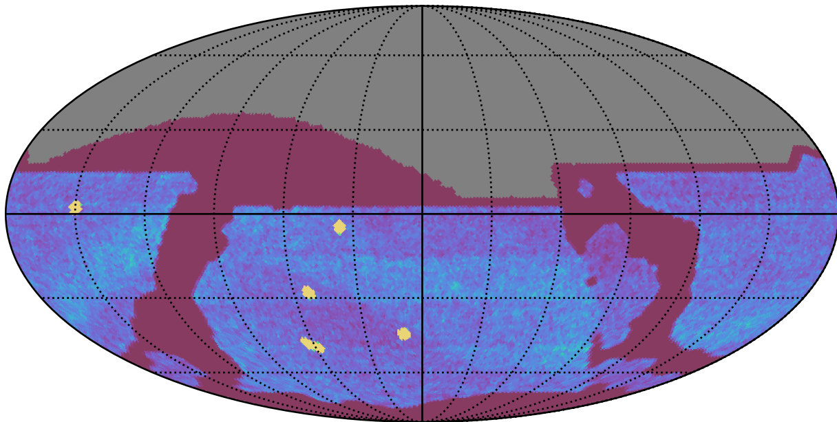
ddf_loaded_fl2_v3.4_10yrs All sky all bands: NVisits
