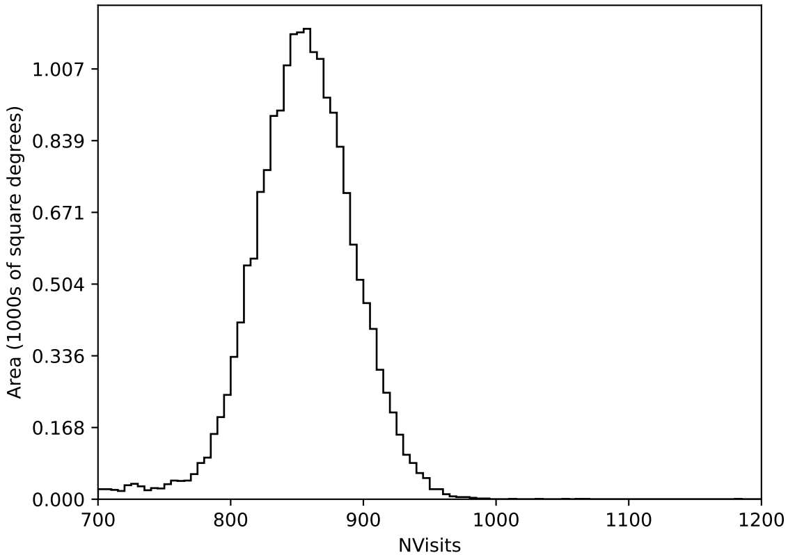
ddf_loaded_fl2_v3.4_10yrs All sky all bands: NVisits
