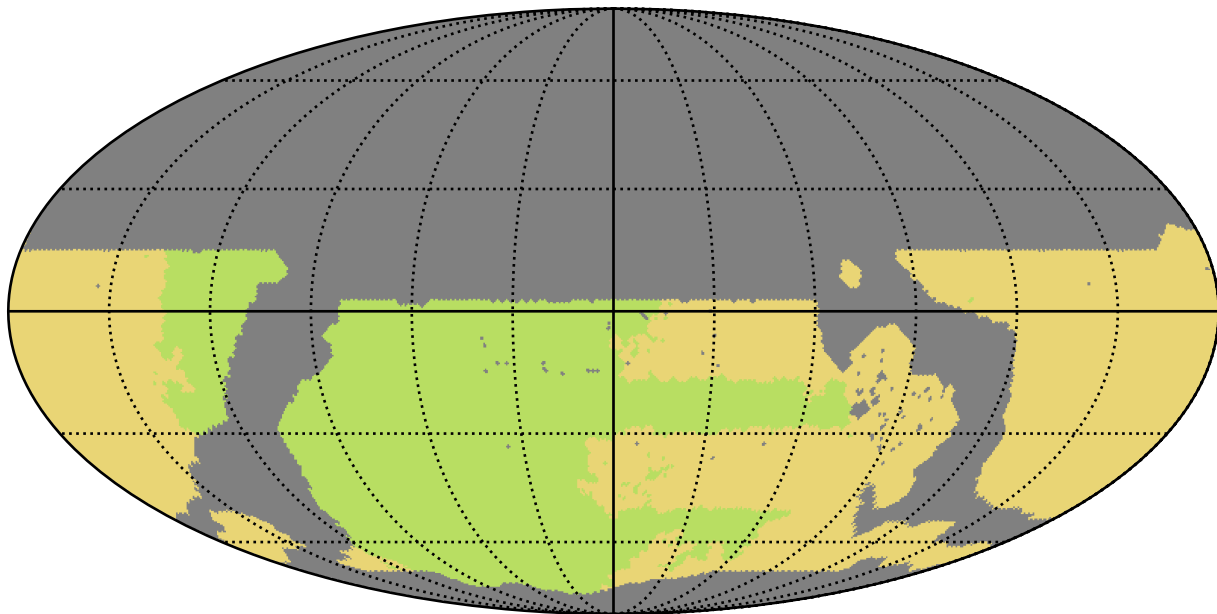
ddf_loaded_fl2_v3.4_10yrs WFD all bands: NSeasons
