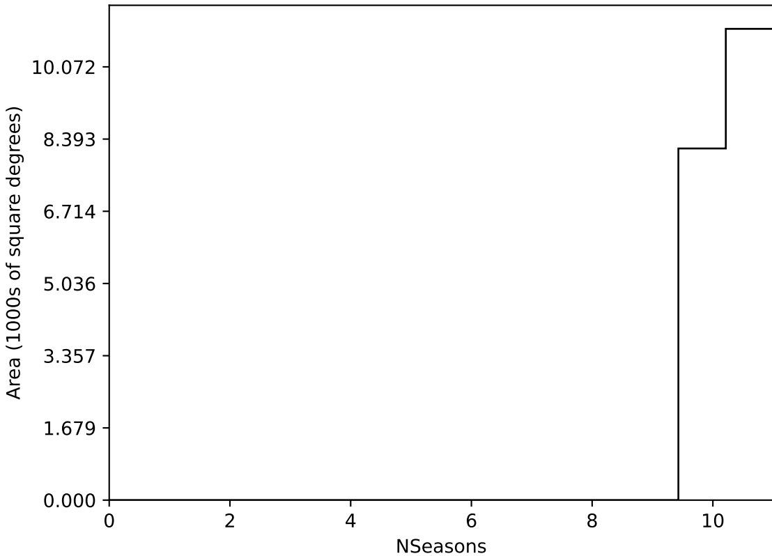
ddf_loaded_fl2_v3.4_10yrs WFD all bands: NSeasons
