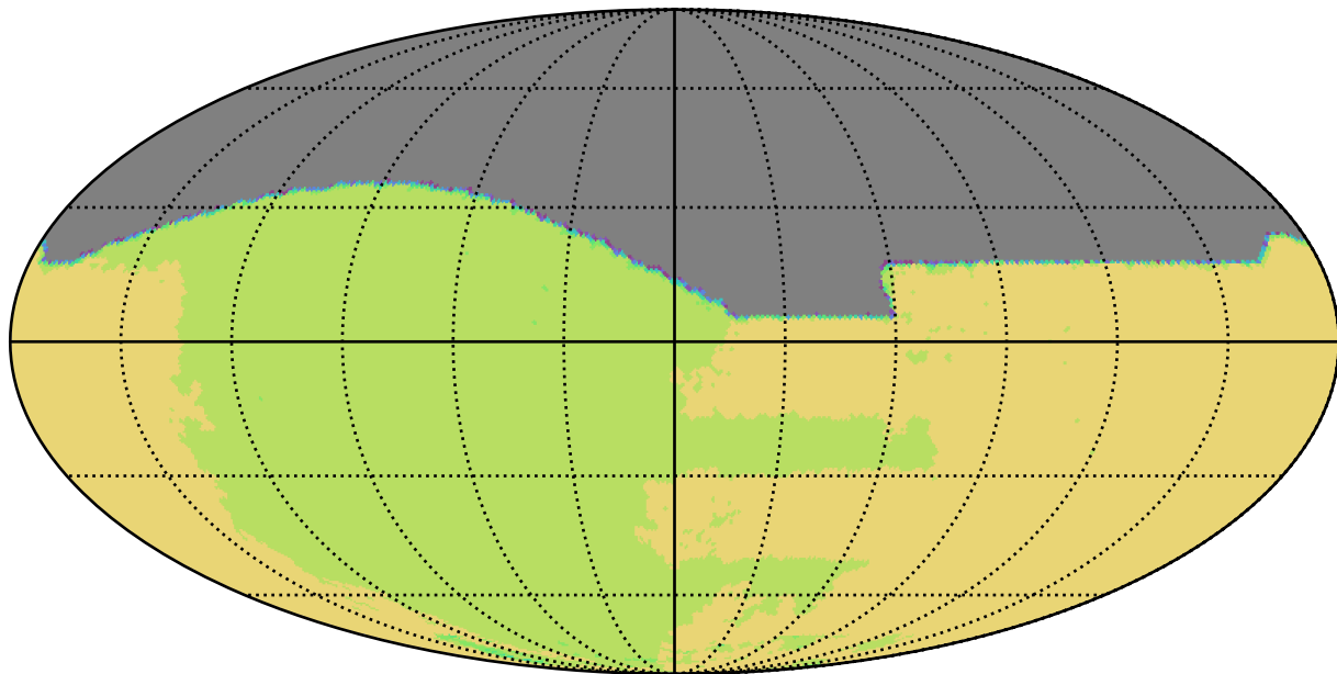
ddf_loaded_fl2_v3.4_10yrs All sky all bands: NSeasons
