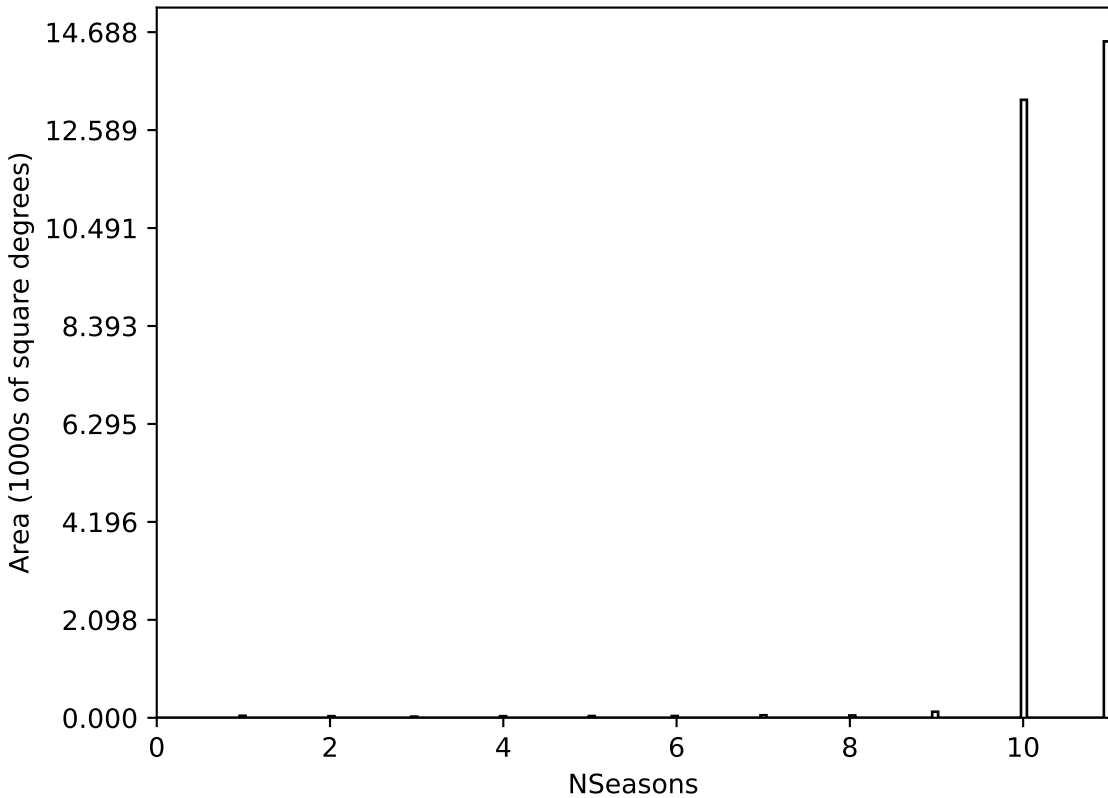
ddf_loaded_fl2_v3.4_10yrs All sky all bands: NSeasons
