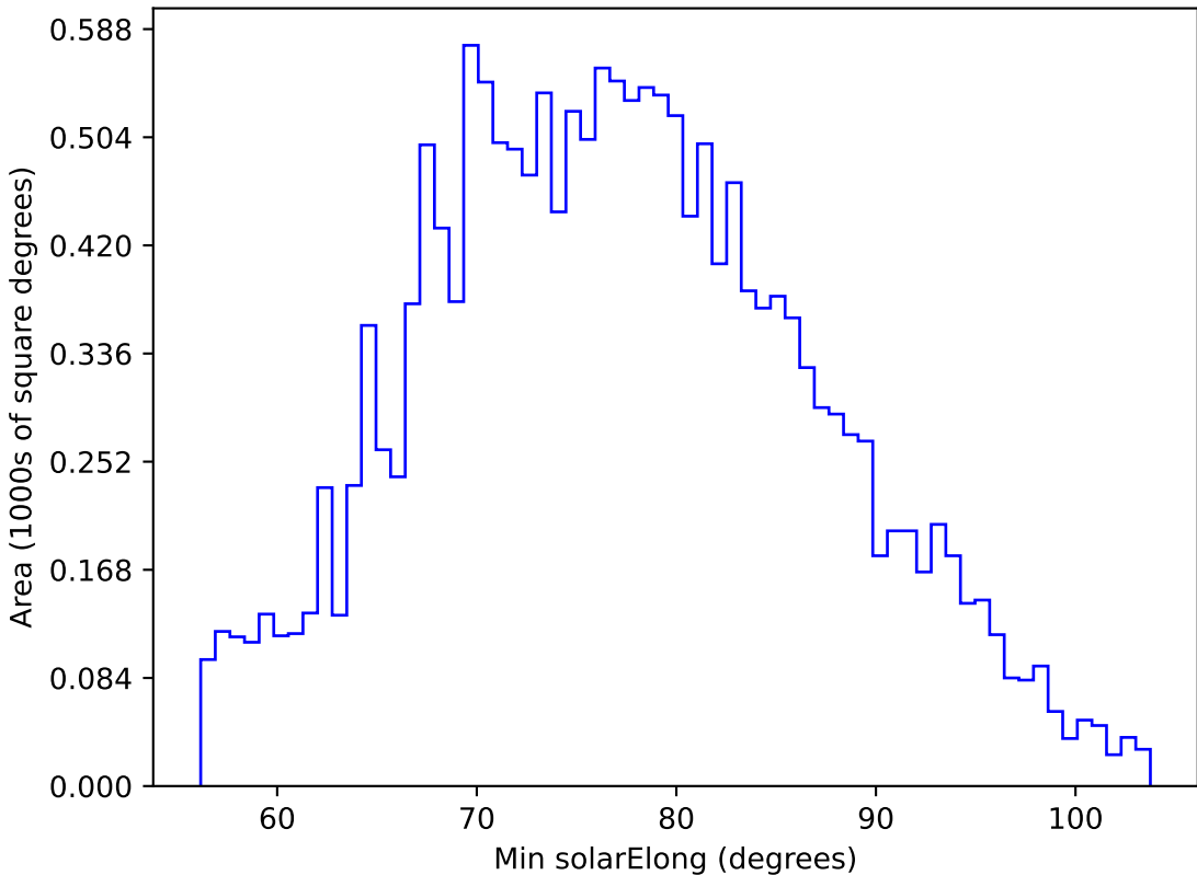
ddf_loaded_fl2_v3.4_10yrs WFD u band: Min solarElong
