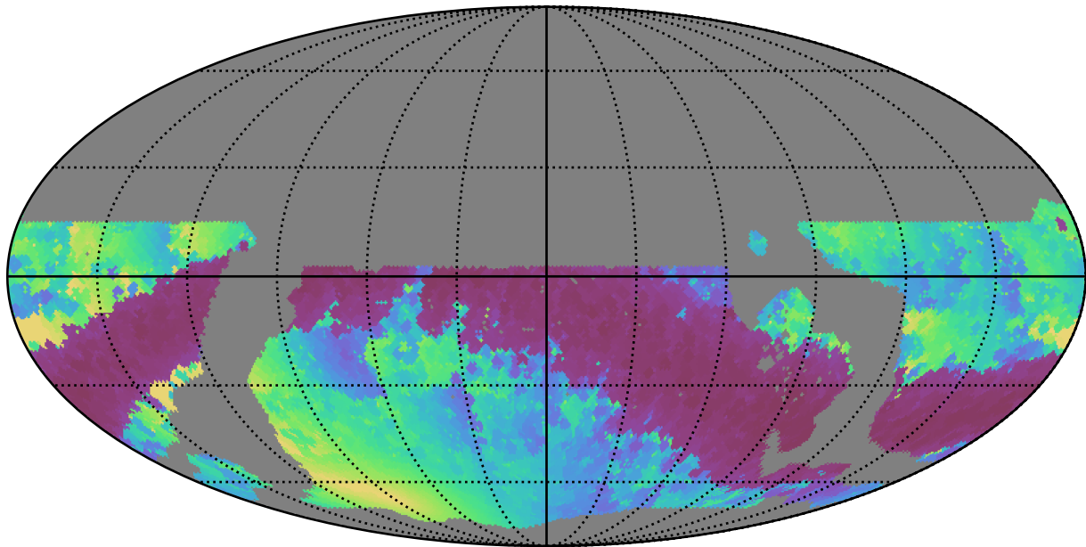
ddf_loaded_fl2_v3.4_10yrs WFD r band: Min solarElong
