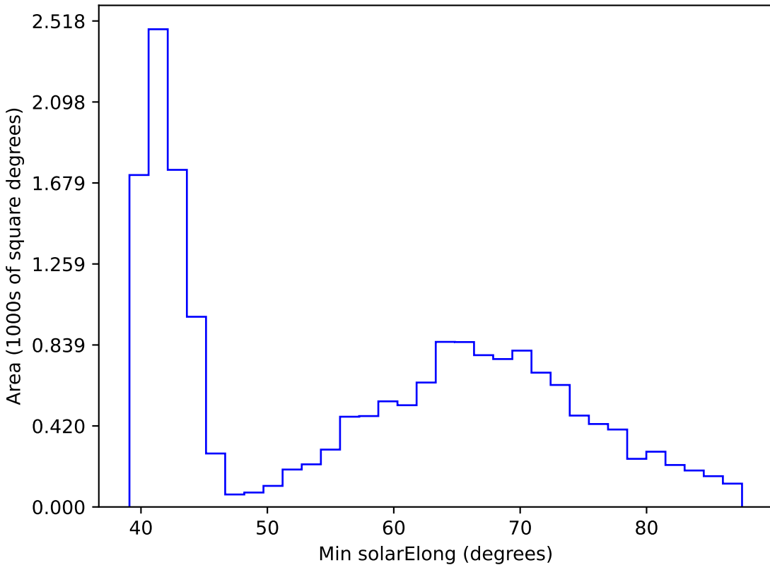
ddf_loaded_fl2_v3.4_10yrs WFD r band: Min solarElong
