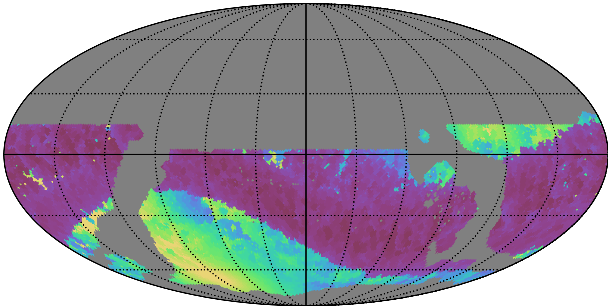
ddf_loaded_fl2_v3.4_10yrs WFD i band: Min solarElong
