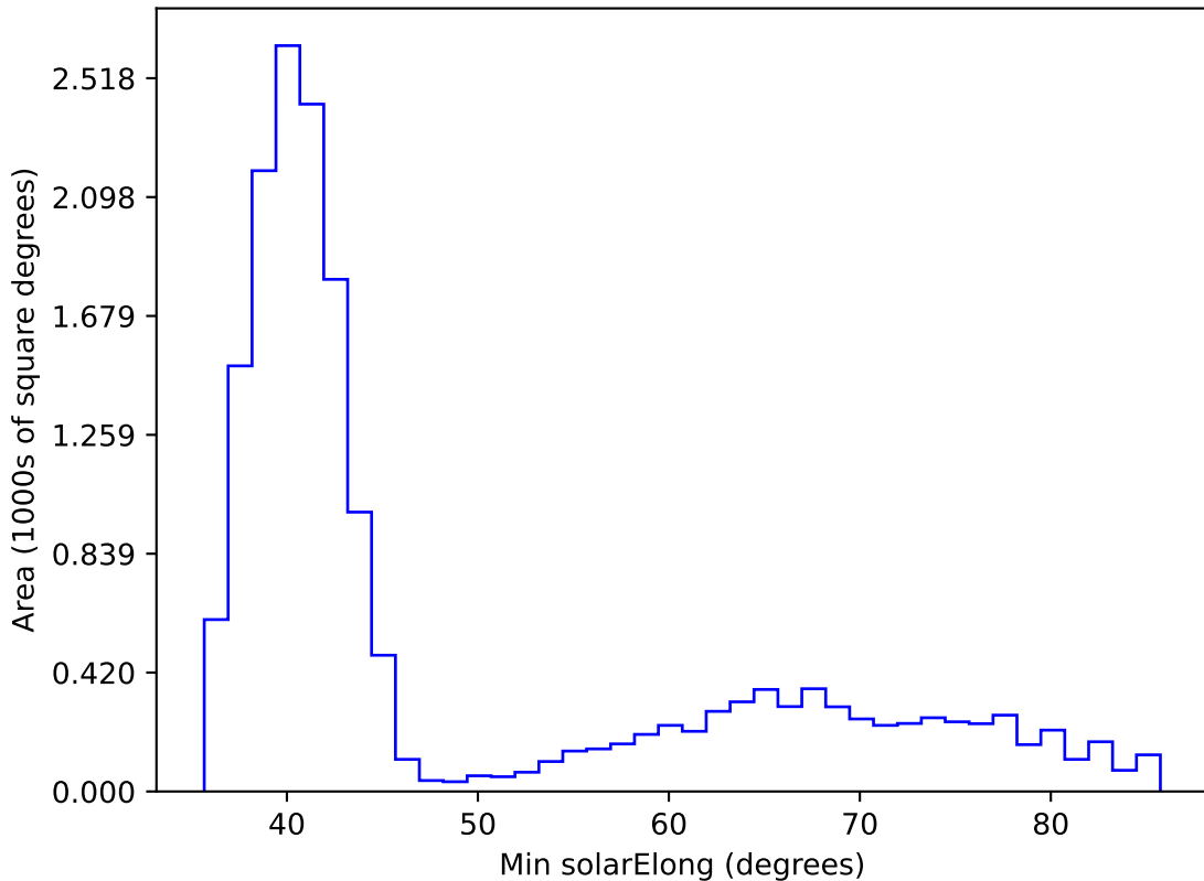
ddf_loaded_fl2_v3.4_10yrs WFD i band: Min solarElong
