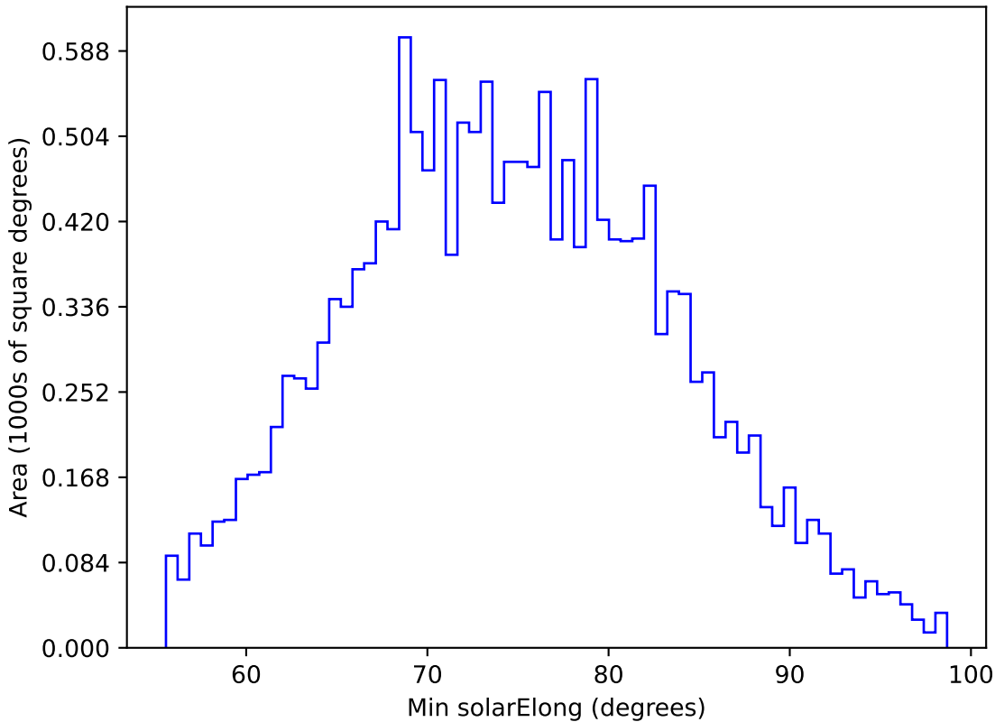
ddf_loaded_fl2_v3.4_10yrs WFD g band: Min solarElong
