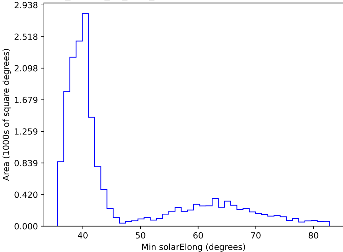
ddf_loaded_fl2_v3.4_10yrs WFD all bands: Min solarElong
