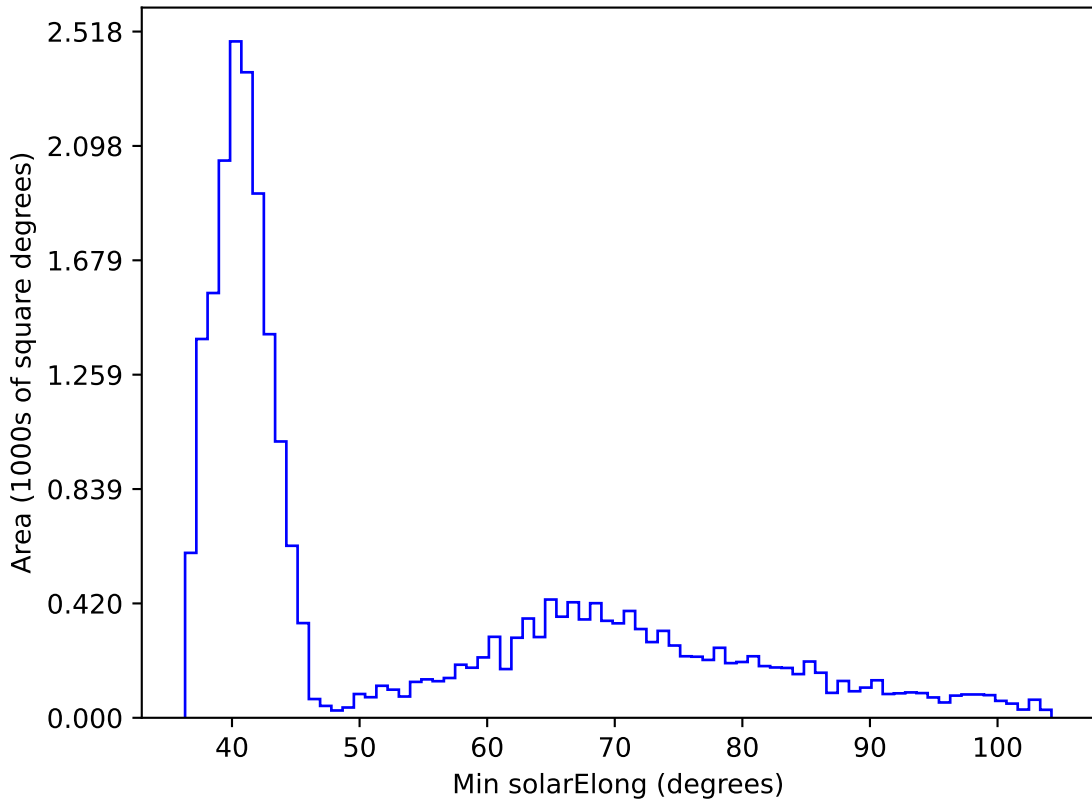
ddf_loaded_fl2_v3.4_10yrs All sky z band: Min solarElong
