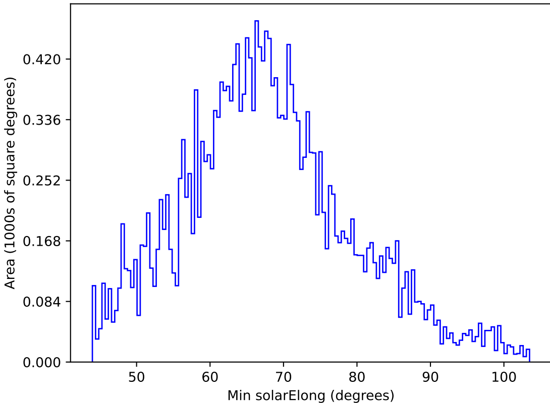
ddf_loaded_fl2_v3.4_10yrs All sky y band: Min solarElong
