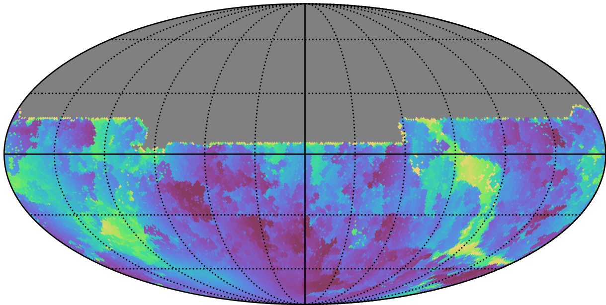
ddf_loaded_fl2_v3.4_10yrs All sky u band: Min solarElong
