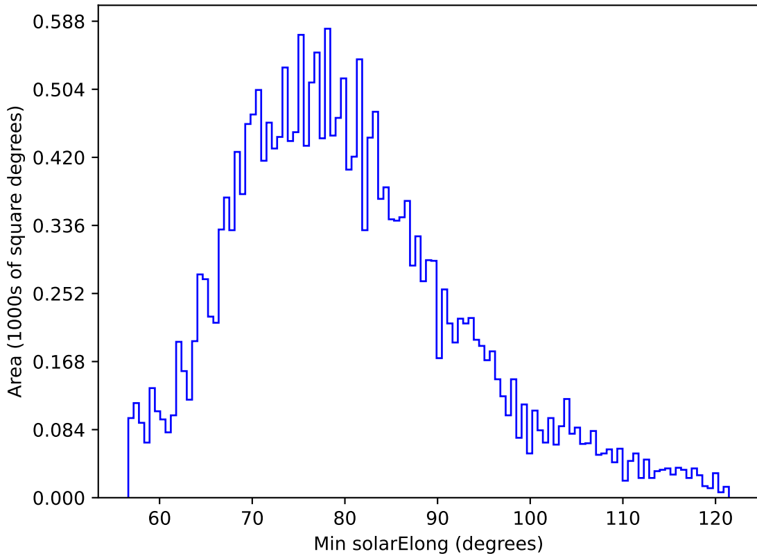
ddf_loaded_fl2_v3.4_10yrs All sky u band: Min solarElong
