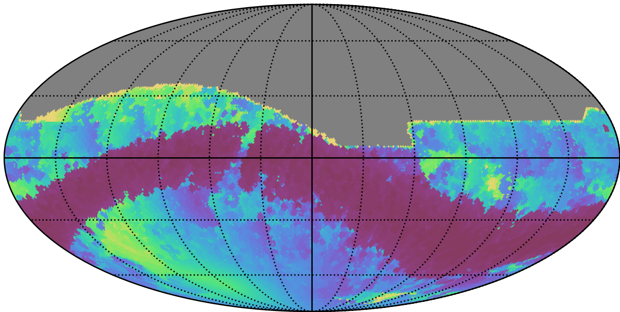
ddf_loaded_fl2_v3.4_10yrs All sky r band: Min solarElong
