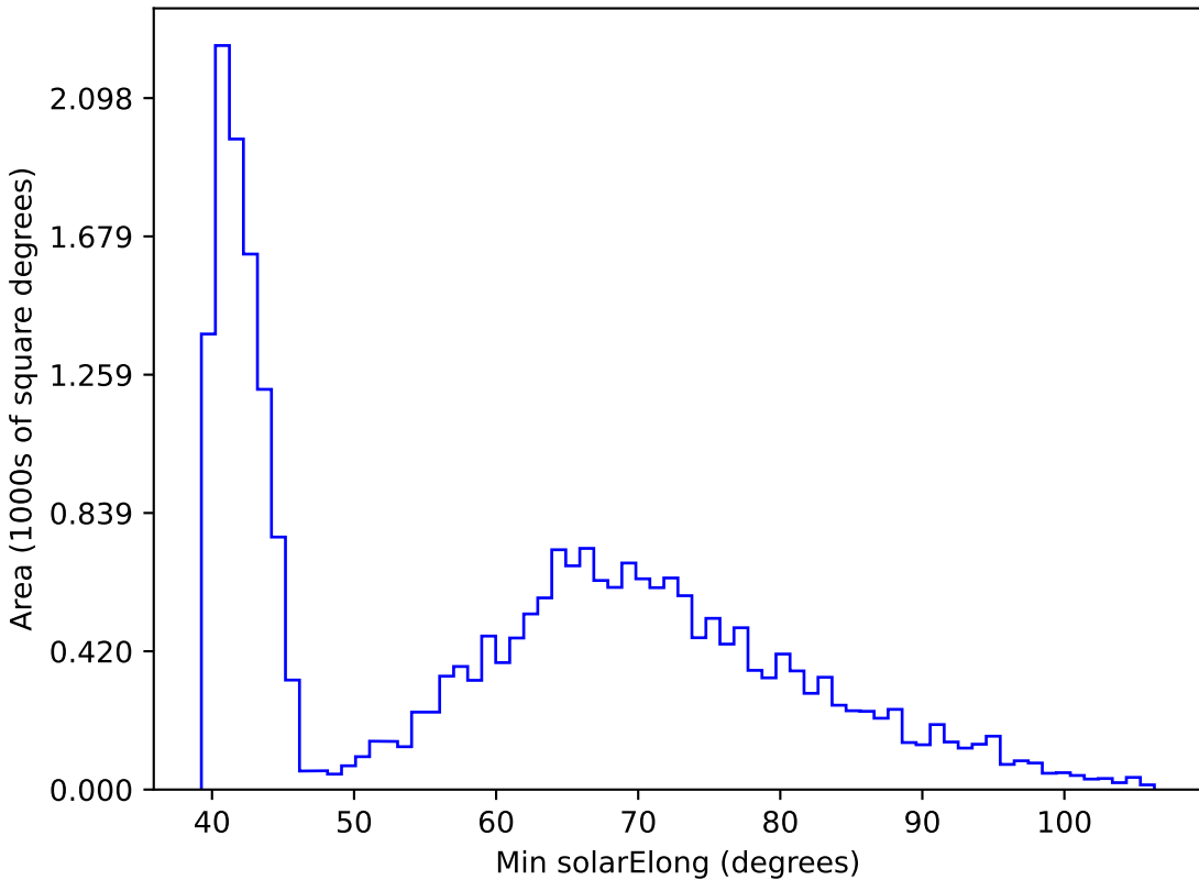
ddf_loaded_fl2_v3.4_10yrs All sky r band: Min solarElong
