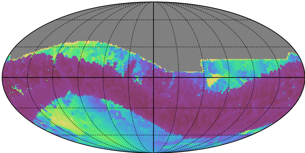
ddf_loaded_fl2_v3.4_10yrs All sky i band: Min solarElong
