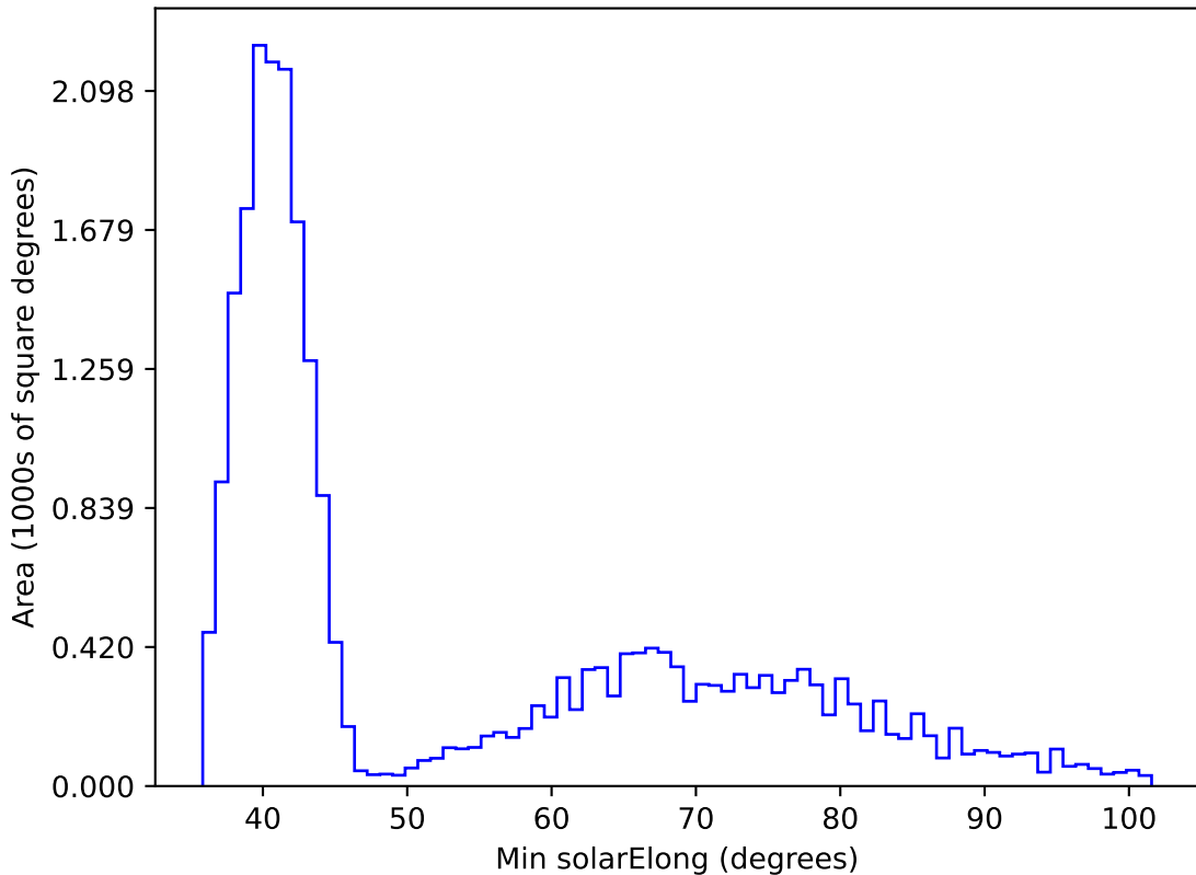
ddf_loaded_fl2_v3.4_10yrs All sky i band: Min solarElong
