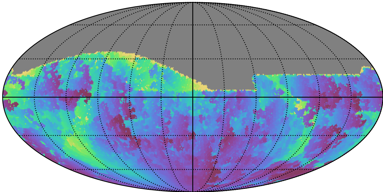
ddf_loaded_fl2_v3.4_10yrs All sky g band: Min solarElong
