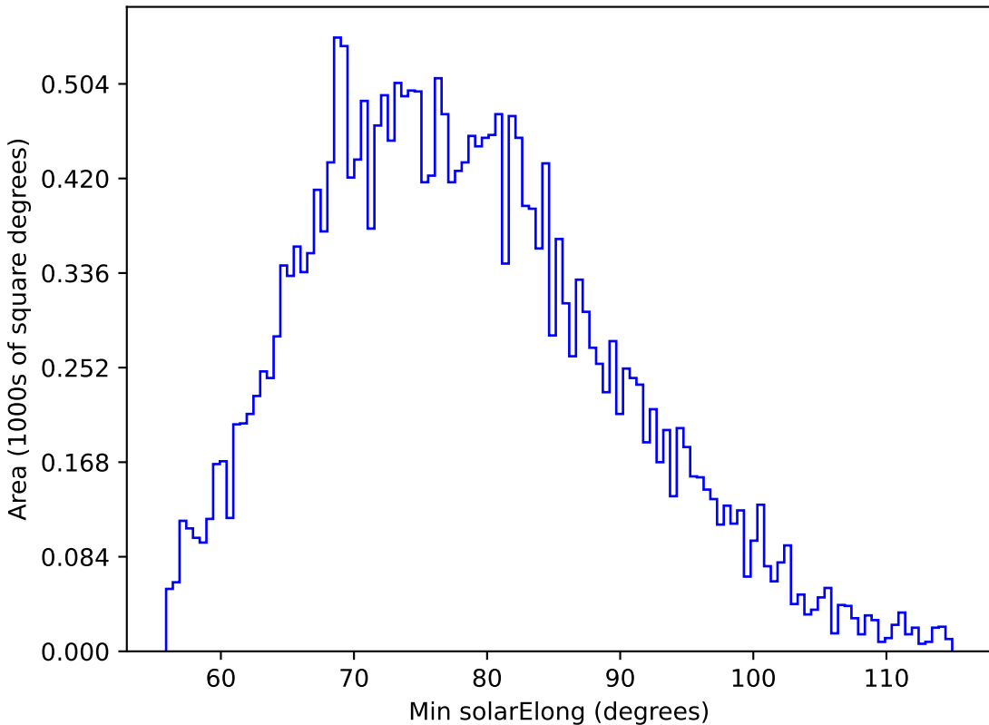
ddf_loaded_fl2_v3.4_10yrs All sky g band: Min solarElong
