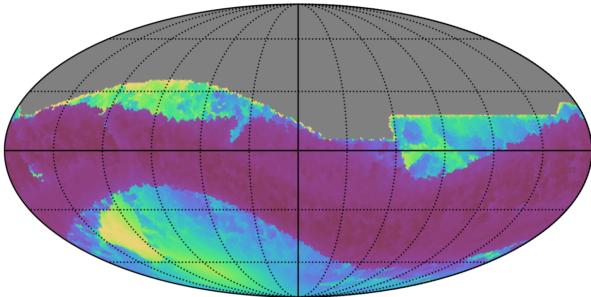
ddf_loaded_fl2_v3.4_10yrs All sky all bands: Min solarElong
