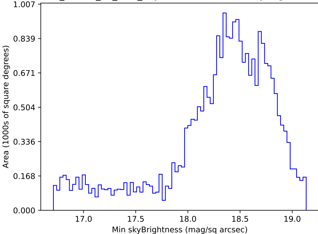
ddf_loaded_fl2_v3.4_10yrs Yr 1 z band: Min skyBrightness
