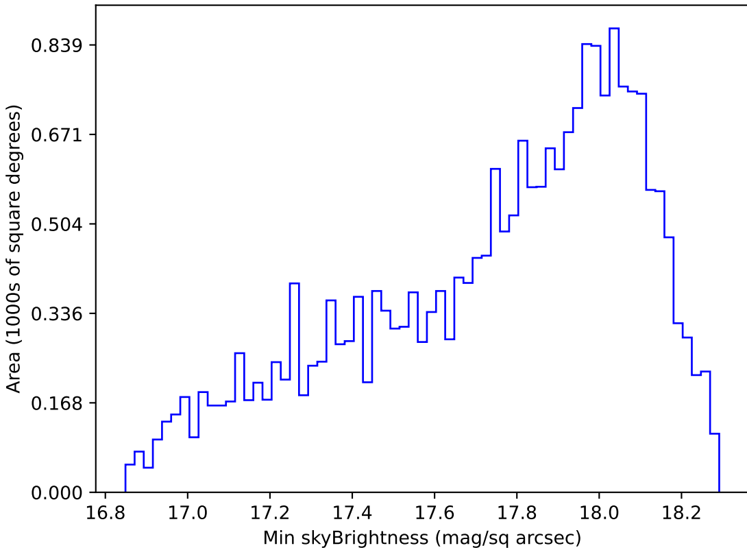
ddf_loaded_fl2_v3.4_10yrs Yr 1 y band: Min skyBrightness
