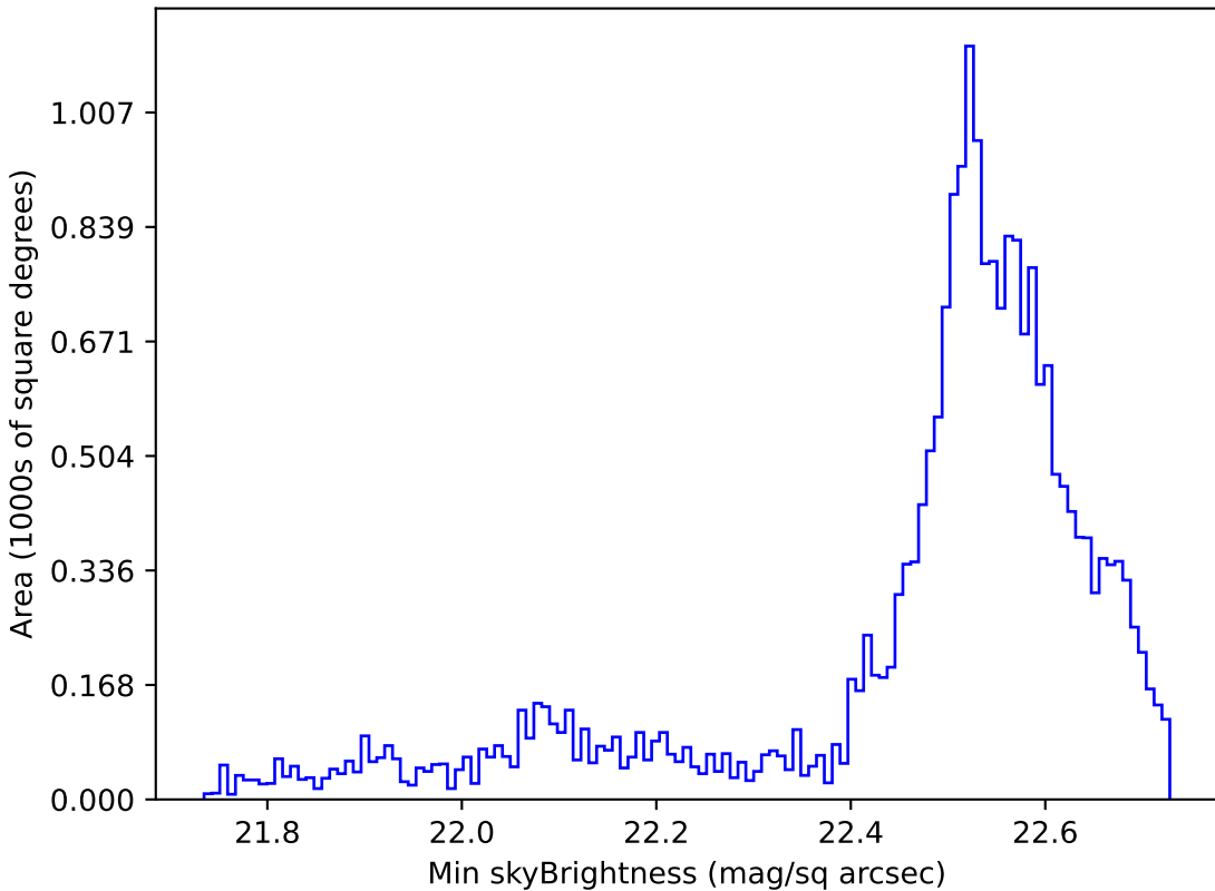
ddf_loaded_fl2_v3.4_10yrs Yr 1 u band: Min skyBrightness
