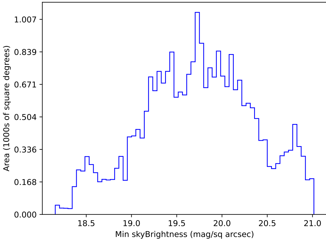
ddf_loaded_fl2_v3.4_10yrs Yr 1 r band: Min skyBrightness
