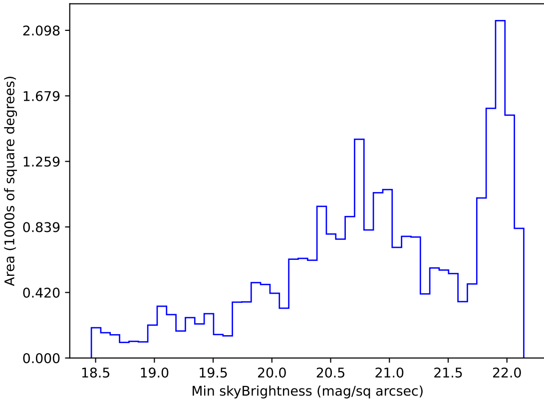
ddf_loaded_fl2_v3.4_10yrs Yr 1 g band: Min skyBrightness
