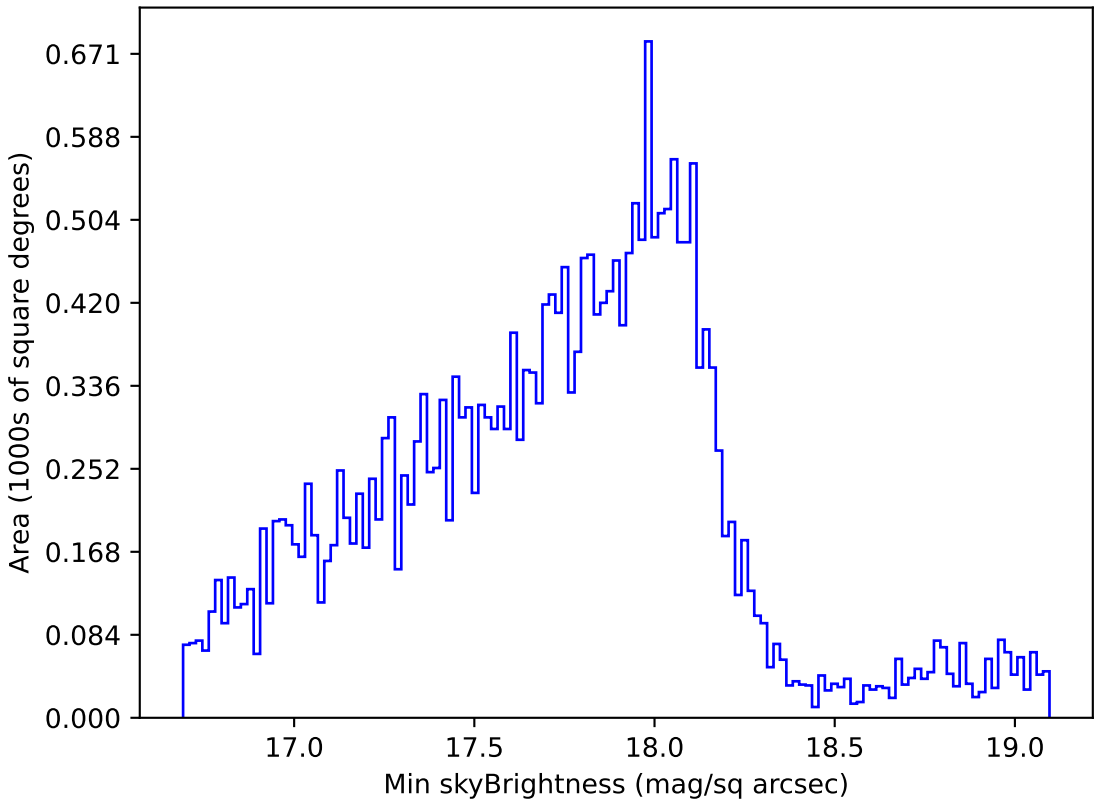
ddf_loaded_fl2_v3.4_10yrs Yr 1 all bands: Min skyBrightness
