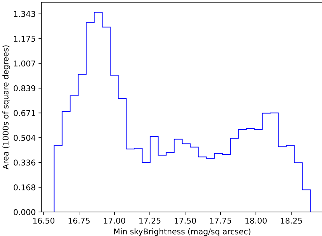
ddf_loaded_fl2_v3.4_10yrs WFD z band: Min skyBrightness
