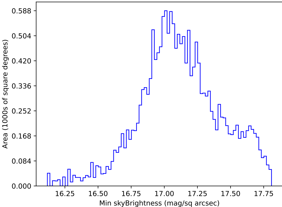
ddf_loaded_fl2_v3.4_10yrs WFD y band: Min skyBrightness
