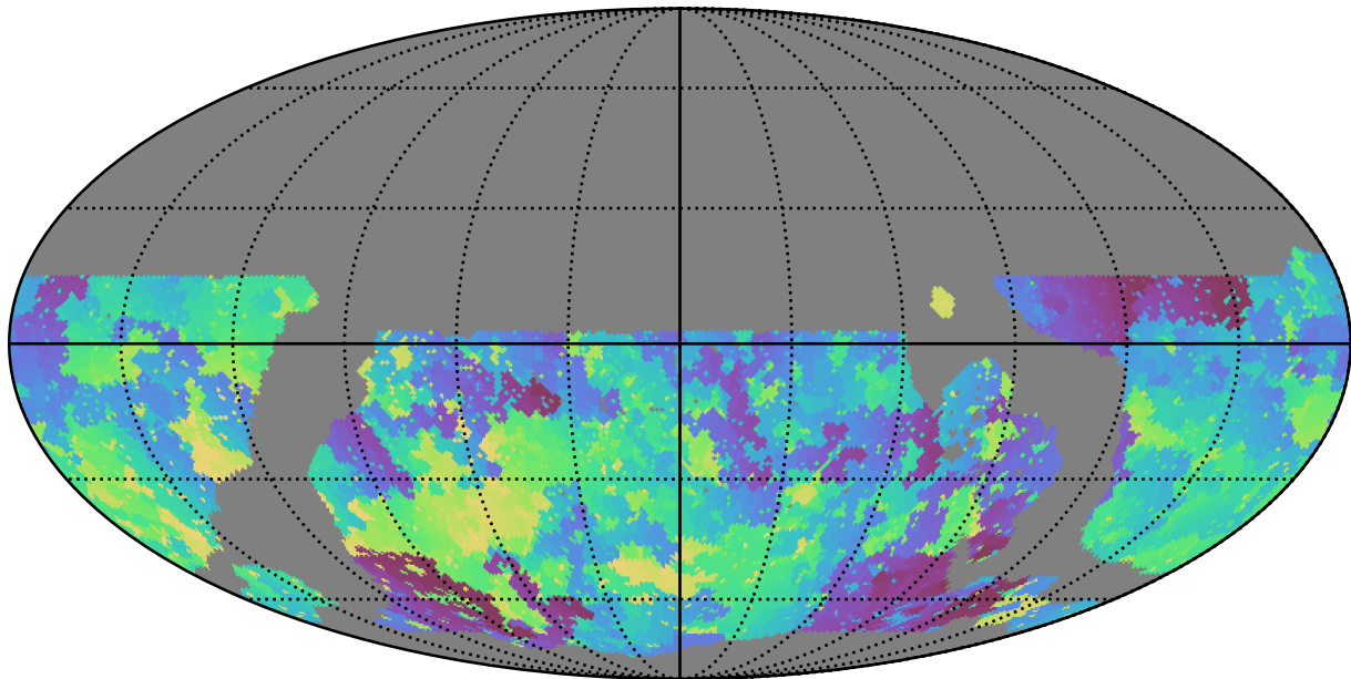
ddf_loaded_fl2_v3.4_10yrs WFD u band: Min skyBrightness
