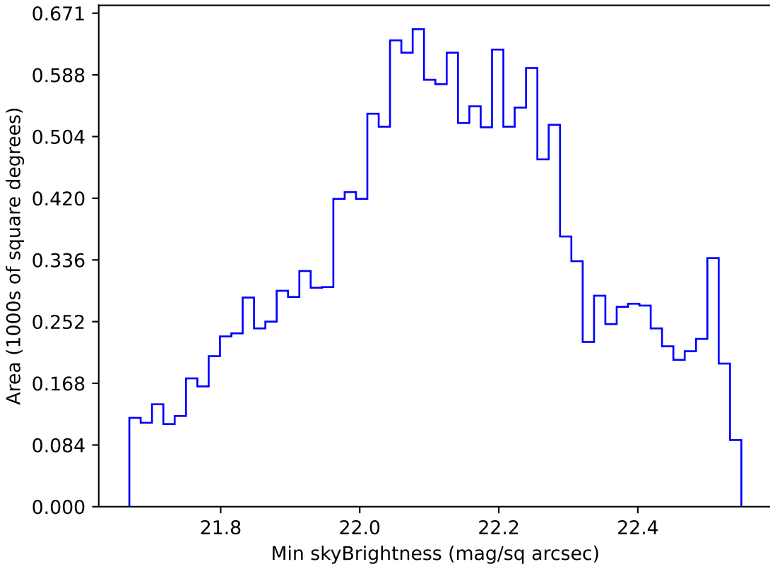
ddf_loaded_fl2_v3.4_10yrs WFD u band: Min skyBrightness
