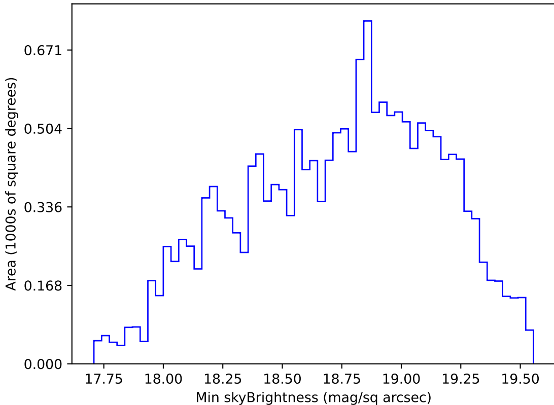
ddf_loaded_fl2_v3.4_10yrs WFD r band: Min skyBrightness
