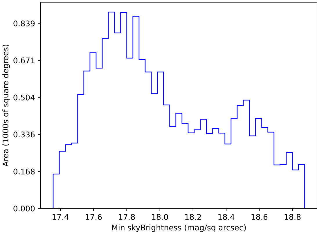
ddf_loaded_fl2_v3.4_10yrs WFD i band: Min skyBrightness
