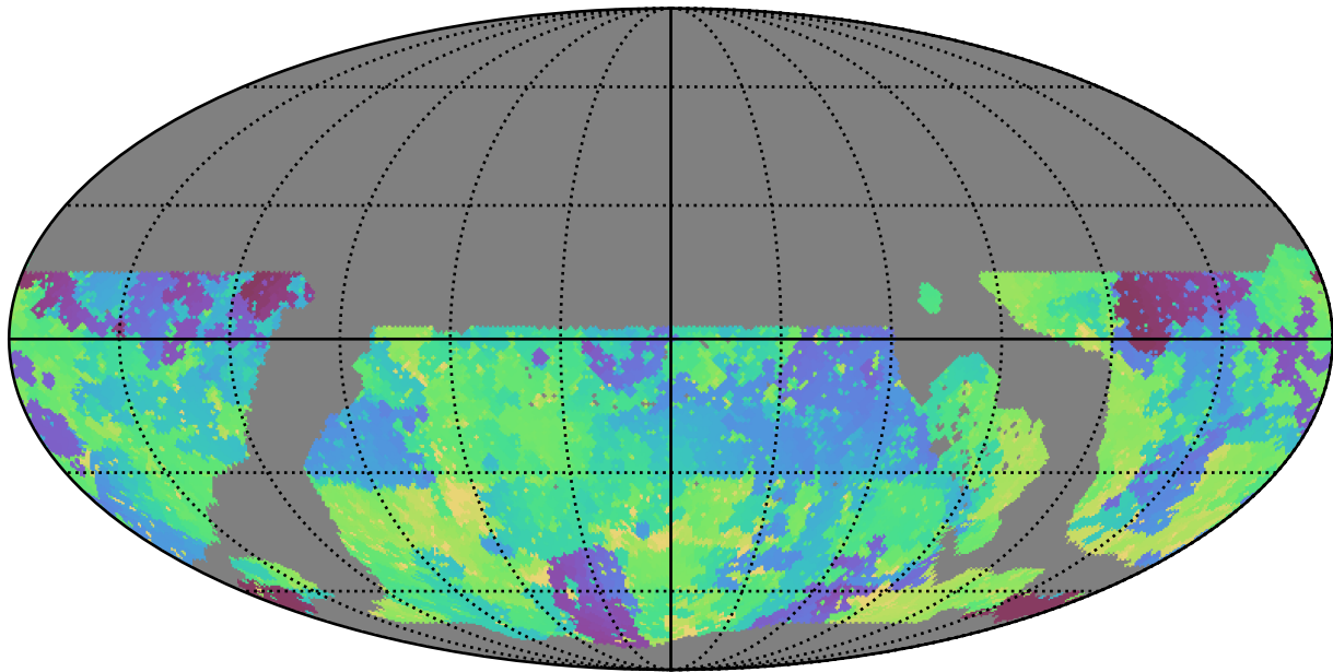
ddf_loaded_fl2_v3.4_10yrs WFD g band: Min skyBrightness
