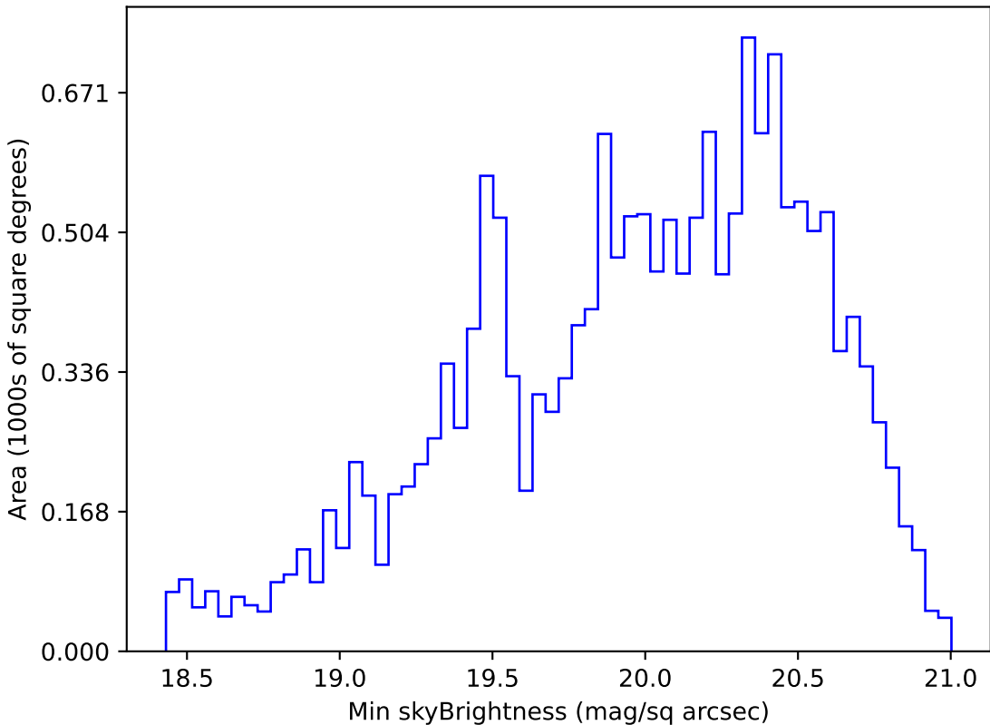
ddf_loaded_fl2_v3.4_10yrs WFD g band: Min skyBrightness
