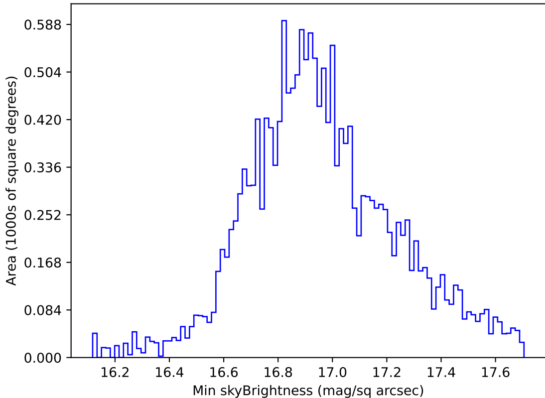
ddf_loaded_fl2_v3.4_10yrs WFD all bands: Min skyBrightness
