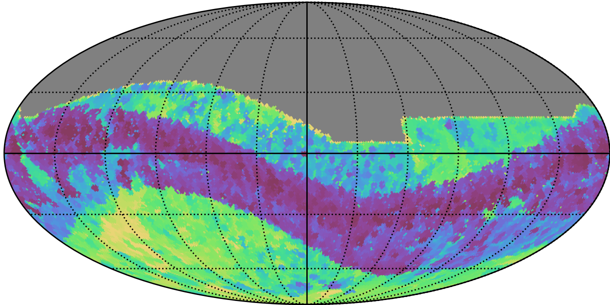
ddf_loaded_fl2_v3.4_10yrs All sky z band: Min skyBrightness
