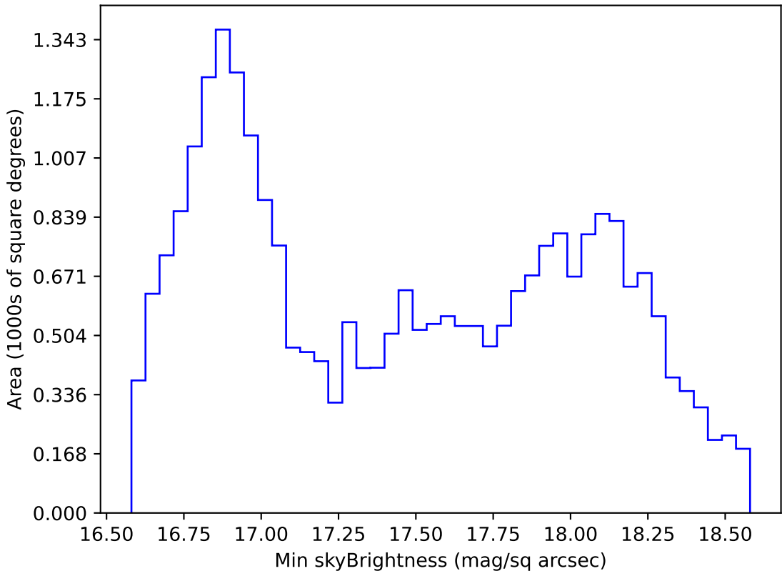
ddf_loaded_fl2_v3.4_10yrs All sky z band: Min skyBrightness
