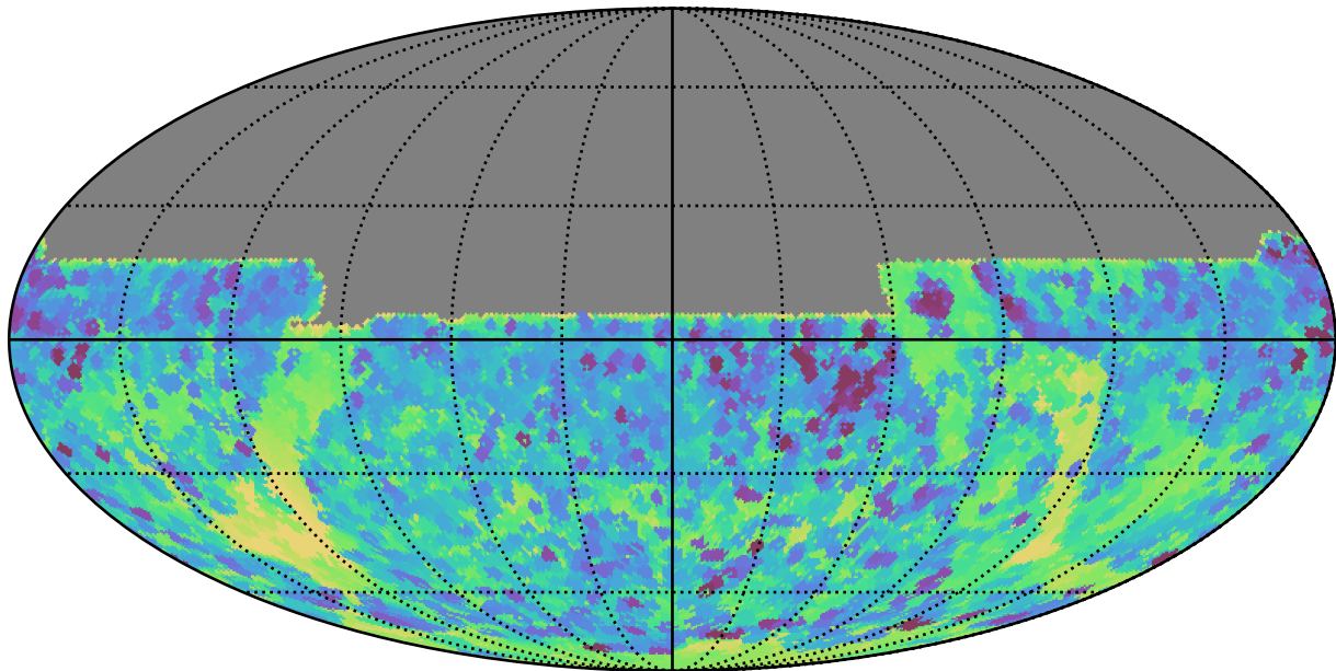
ddf_loaded_fl2_v3.4_10yrs All sky y band: Min skyBrightness
