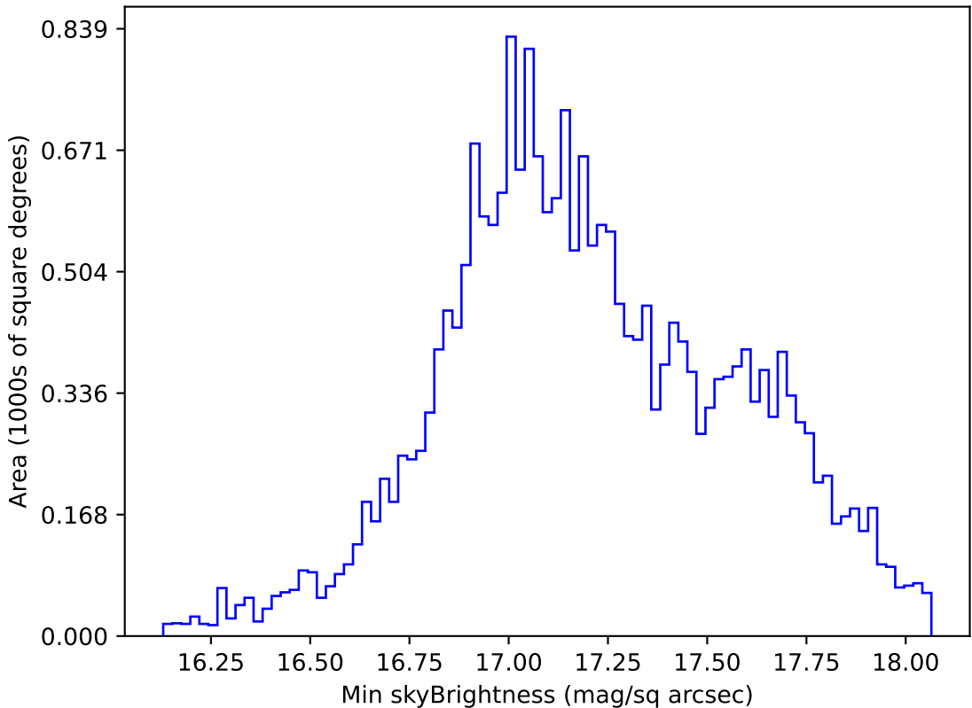
ddf_loaded_fl2_v3.4_10yrs All sky y band: Min skyBrightness
