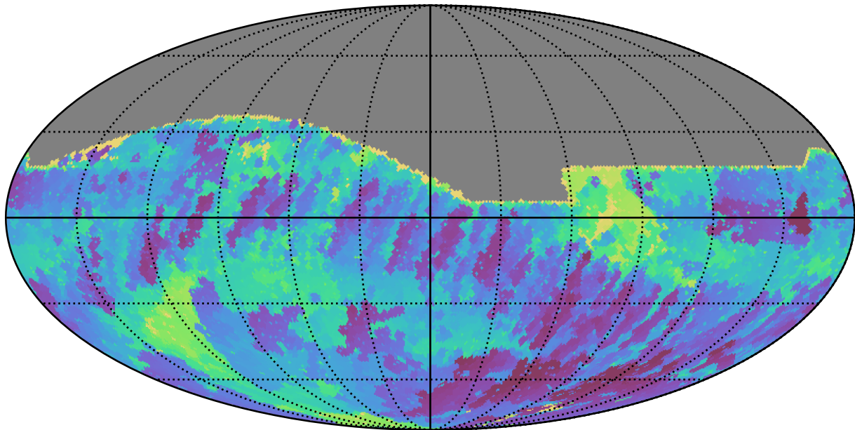
ddf_loaded_fl2_v3.4_10yrs All sky r band: Min skyBrightness
