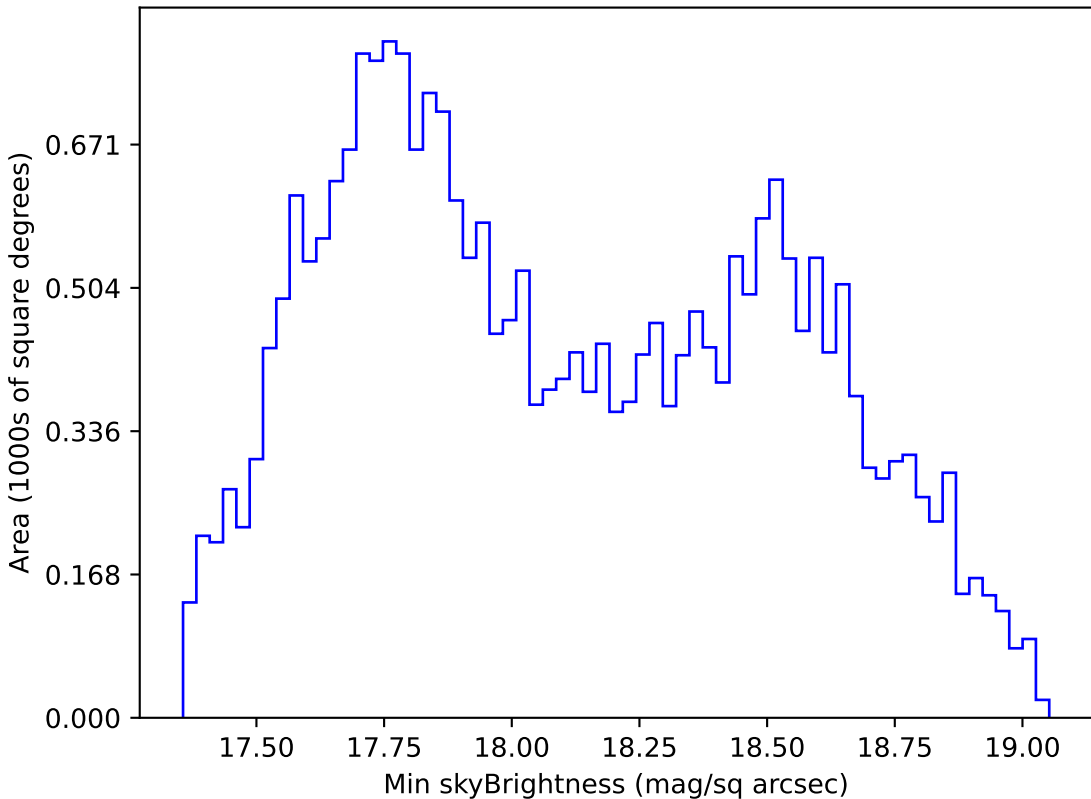
ddf_loaded_fl2_v3.4_10yrs All sky i band: Min skyBrightness
