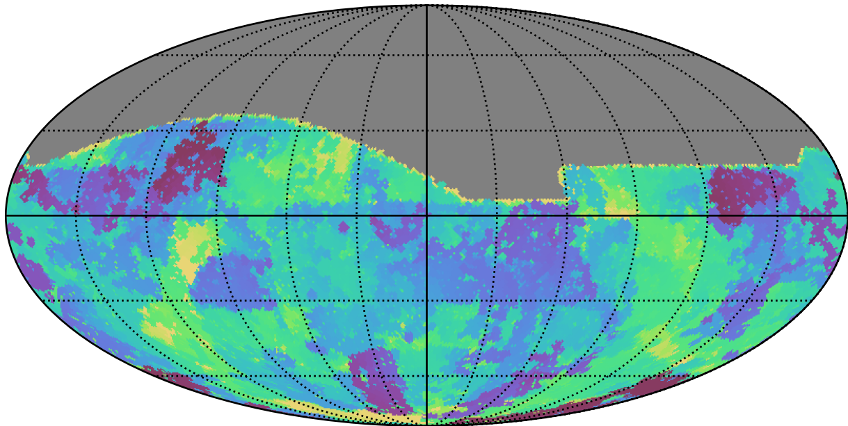
ddf_loaded_fl2_v3.4_10yrs All sky g band: Min skyBrightness
